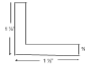
Blunt Nose (Rectangle) edge trim _____
